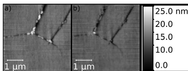
Figure 8. HS-AFM frames showing grain boundaries in sensitised stainless steel under a droplet of deionised water with 5 \text{ mg L}^{-1} \text{ Cl}^{-} : (a) before and (b) after polarisation. Each 1-megapixel was collected in 0.5 s.
