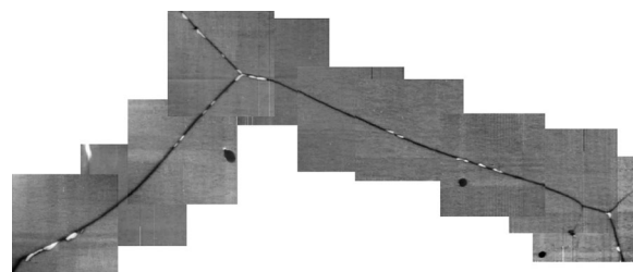
Figure 7. Mosaic of HS-AFM scans showing microstructure of a thermally sensitised 20Cr-25Ni-Nb stabilised stainless steel specimen (C-ring) cross section.
