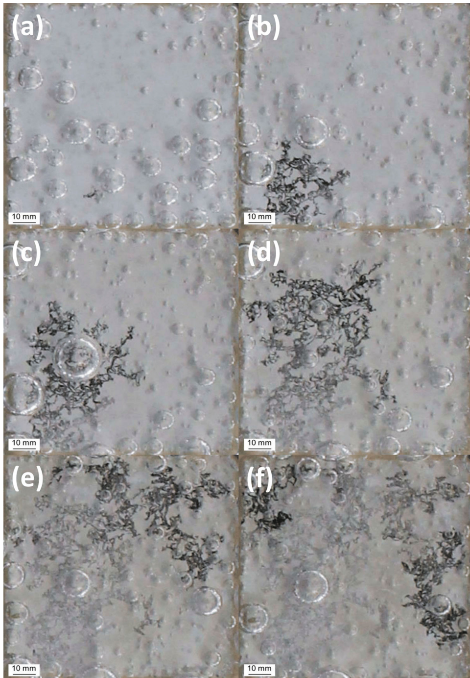
Figure 3. Photographic images showing the extent of corrosion on a Magnox alloy specimen, immersed in aerated 2.5% w/v NaCl (aq) at pH 7, for: (a) 3 h, (b) 6.5 h, (c) 8.7 h, (d) 11 h, (e) 16.7 h, and (f) 19 h.
