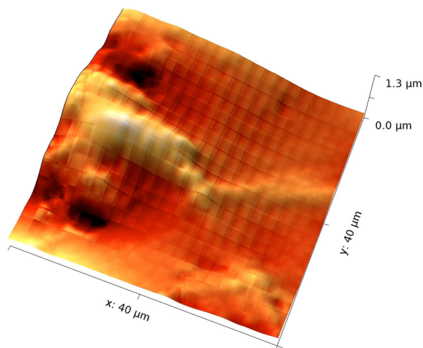
Figure 9. A composite HS-AFM topography map of a Magnox alloy specimen. A filament of filiform-like corrosion product can be seen passing from left to right. Just to the left of the frame was a large pit with dimensions too deep to image using this technique. The 50 mega-pixel image was collected in 100 s.
