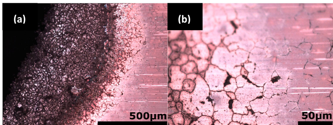
Figure 6. Micrographs of the haematite–metal interface following immersion for 24 h in 1 \text{ mol L}^{-3} NaCl in freely corroding conditions.
