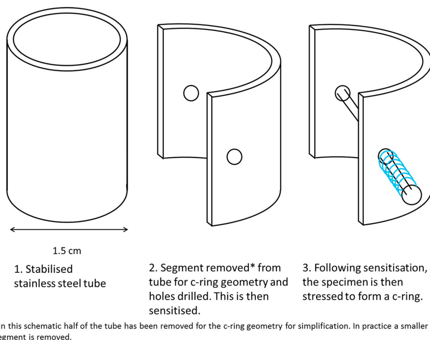
Figure 1. Preparation processes for C-rings.
