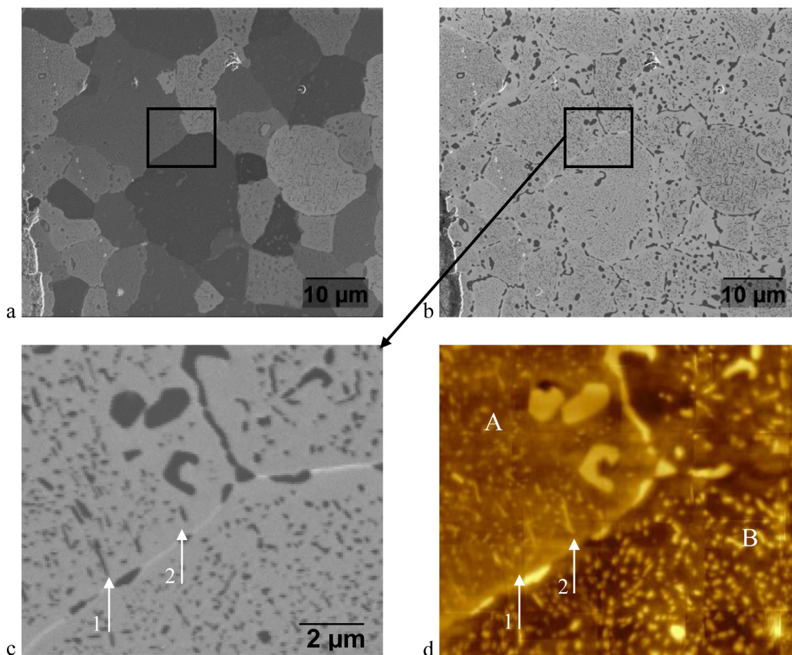
Fig. 3. (a) FIB induced secondary electron micrograph from sample A showing ion channelling contrast. (b) FIB induced secondary electron micrograph of the same area after introduction of XeF 2 gas. (c) Magnified region from image b. (d) Composite HS-AFM image from same area as c) (topographical height colour coded, 30 nm range). The FIB images were acquired after the HS-AFM images.
